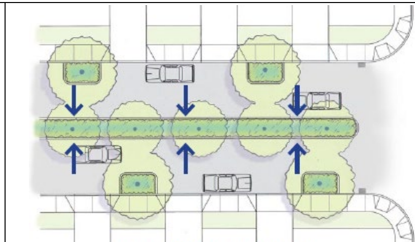
Figure B-2. Reverse Crowned Street Profile. A reversed crowned street is the opposite of a crowned street and directs runoff to the center line of the street. GI facilities may be considered in the median.
