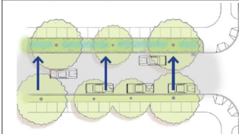
Figure B-3. Side Shed Street Profile. Side shed streets are designed to shed all water to one side of the street. GI facilities would be located on the downslope side.
